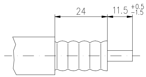
cable trimming
